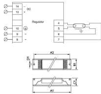
Specifications Philips HF-R 136 TL-D EII 220-240V for 1x36W
